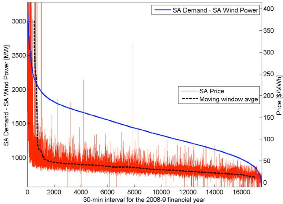
Figure 8: SA Demand minus SA total wind power duration curve for 2008-9 with the corresponding price and moving average price (999 data points per window)
