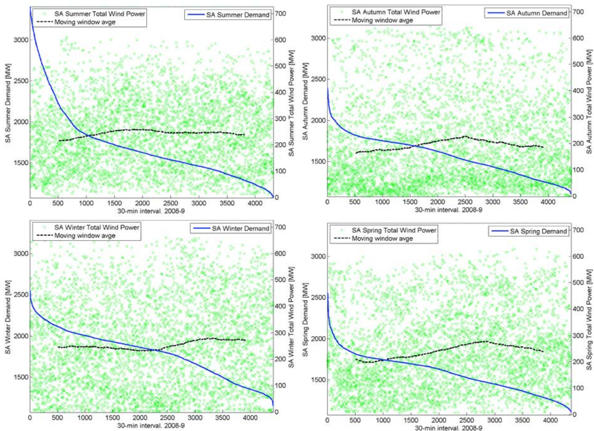
Figure 15: Demand duration curves for each season in 2008-9 with the corresponding total wind power and moving average total wind power (999 data points per window)
