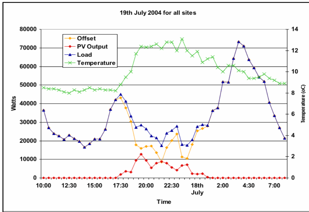
Figure 19 Total Load, PV Output, Offset and Temperature for 19 th July 2004 for all 30 sites
