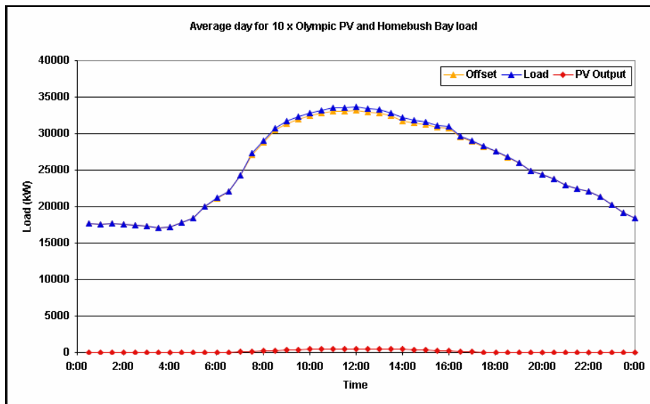
Figure 5 Annual average daily load, estimated PV output and residual load (offset) for Homebush Bay – July 2004 to June 2005
