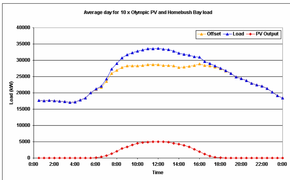
Figure 6 Annual average daily Homebush Bay load and estimated PV contribution if 10x current PV were installed – July 2004 to June 2005
