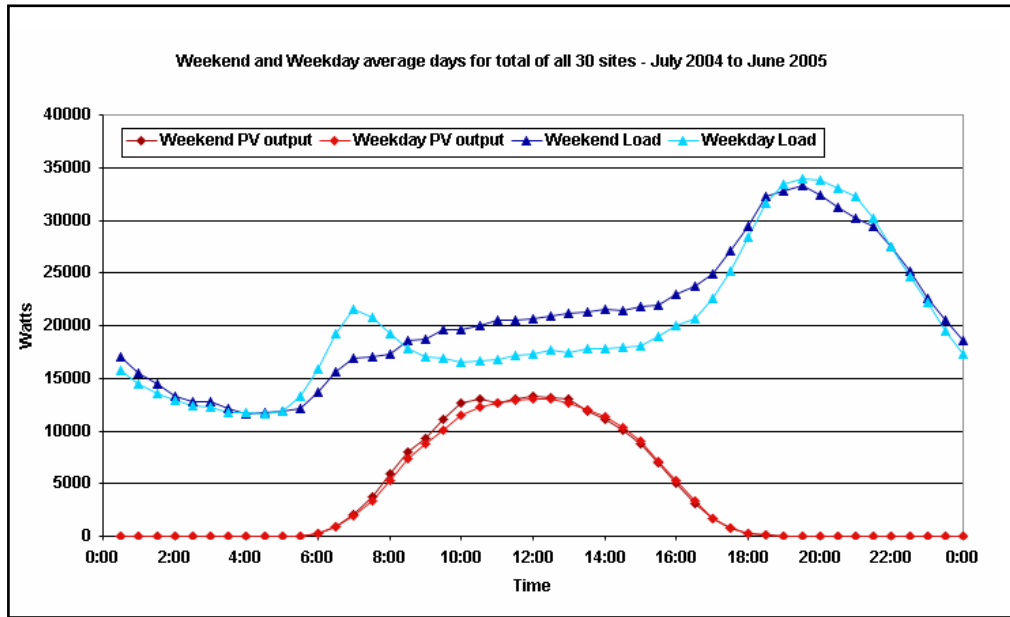
Figure 8 Weekend and weekday average annual daily PV output and load for the total 30 monitored sites - July 2004 to June 2005
