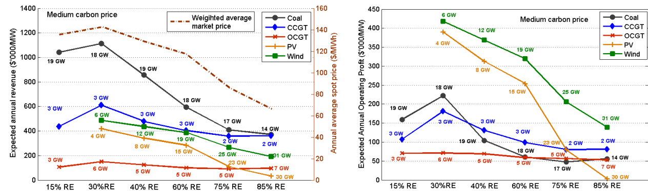
Figure 2. Expected annual revenue, average market price and operating profits of each technology for different renewable penetrations. The installed capacity of each technology is also shown on the graphs.
