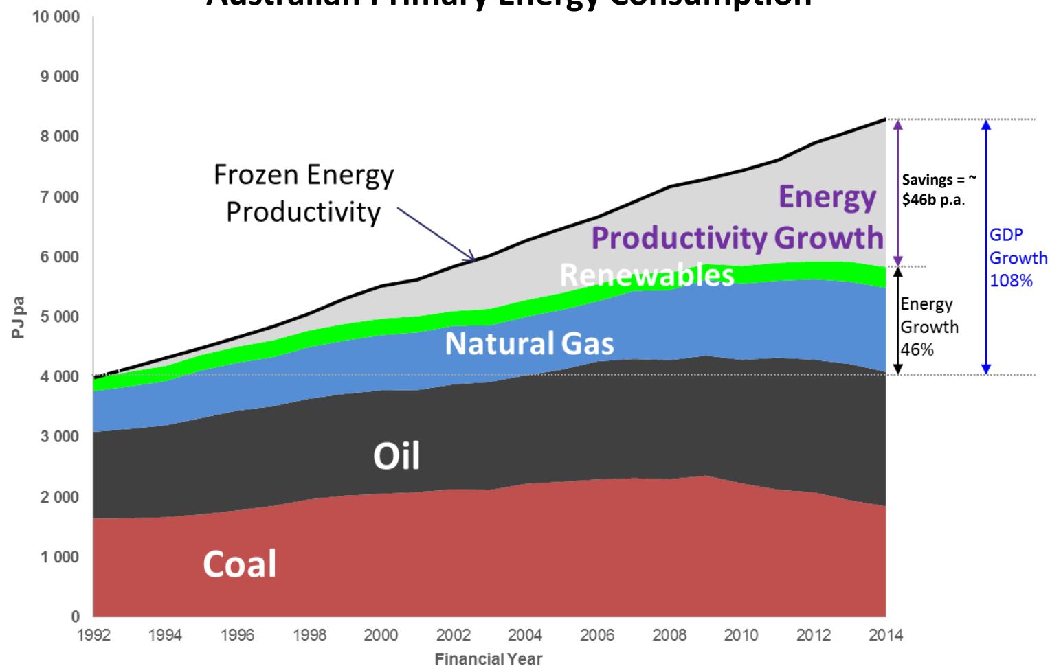
Australian Primary Energy Consumption
